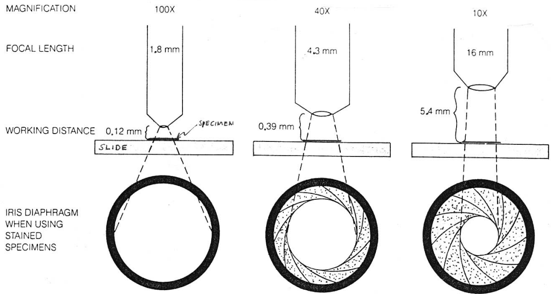
The Relationship between the Working Distance of an Objective Lens and the Adjustment of the Iris Diaphragm
